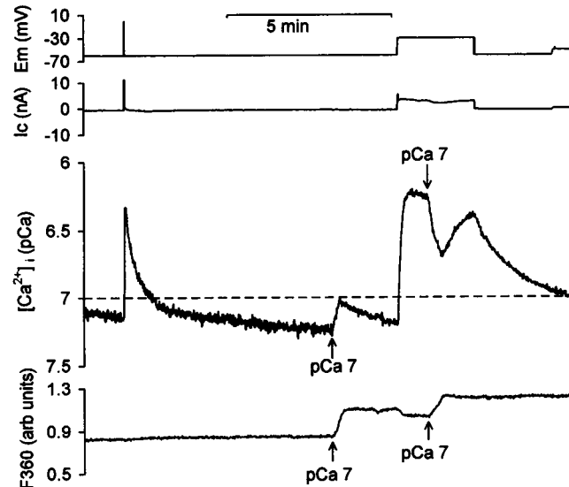
FIGURE 5 The effects of injecting pCa 7 calcium calibration solution at resting and raised [Ca^{2+}]_i levels. Initial depolarization for 1 s to 0 mV. [Ca^{2+}]_i was raised using a sustained (approximately 2 min) depolarization to -30 mV. Arrows indicate the injection of calcium calibration solution. For clarity, the clamp current is shown between -10 and 10 nA.
