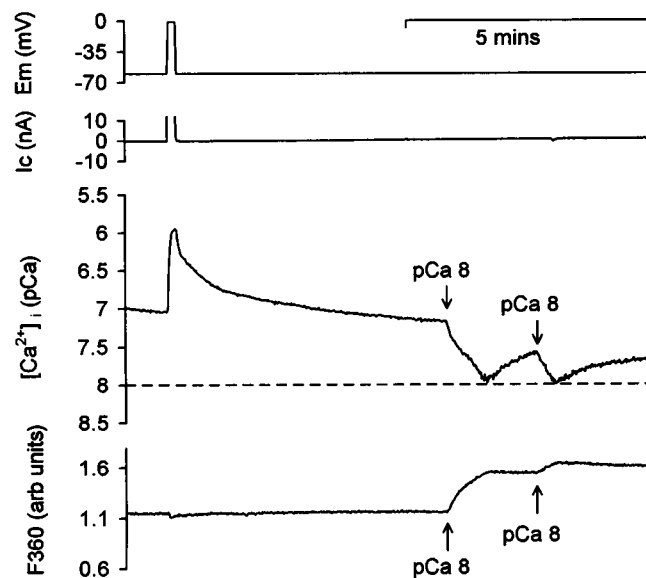
FIGURE 4 The effects on [Ca^{2+}]_i of a 10-s depolarization and injecting pCa 8 calibration solution. Depolarizations for 10 s to 0 mV. For clarity clamp current is only shown between -10 and 10 nA. The arrows indicate the injection of pCa 8 calibration solution.
